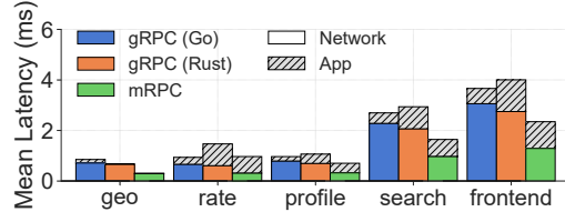
Figure 13: DeathStarBench: Mean latency of gRPC without proxy and mRPC.
